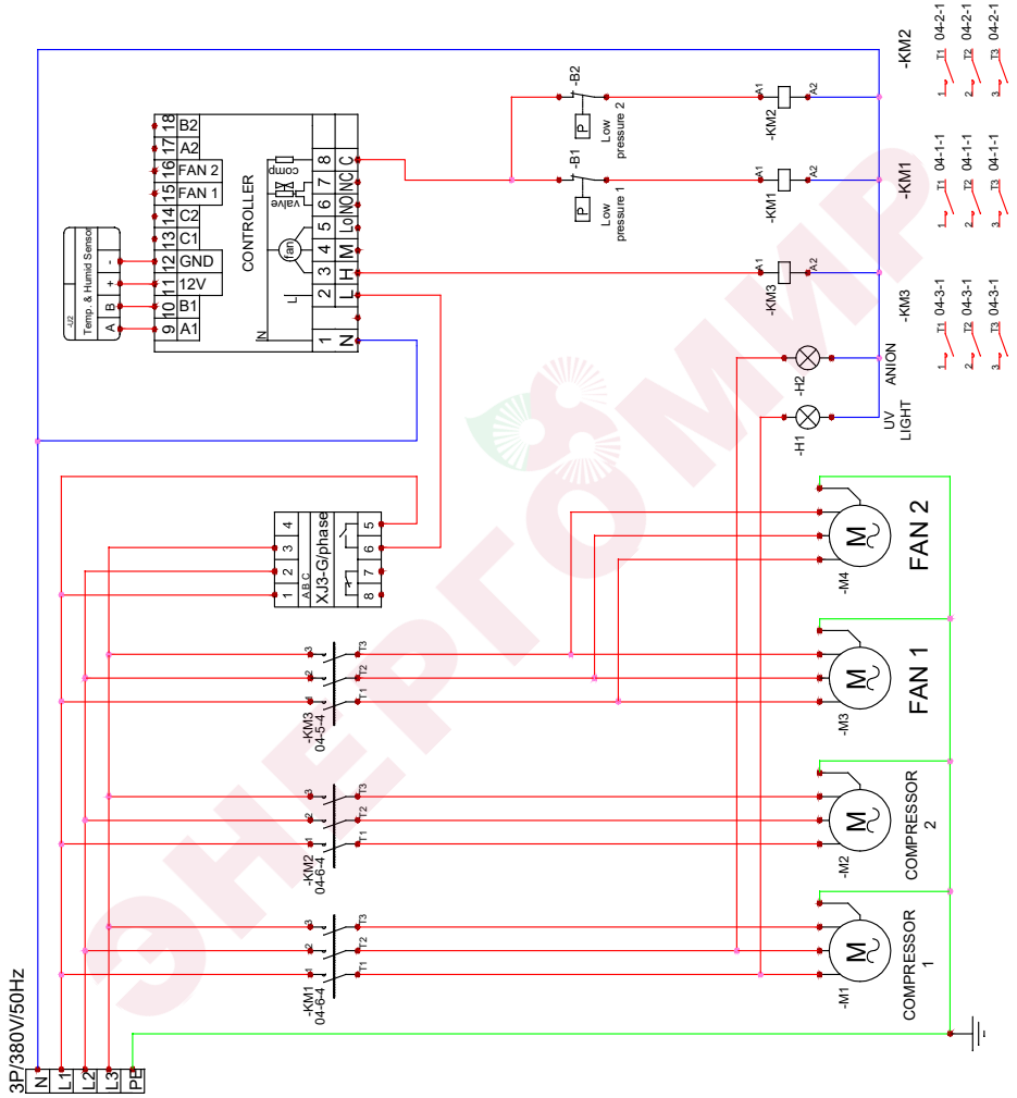
DanVex DEH-3K DEHUMIDIFIER WIRING DIAGRAM
